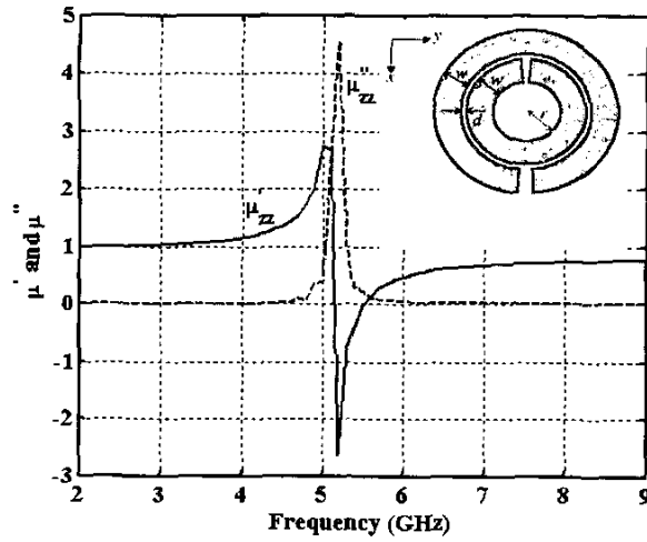
Fig.1 Negative permeability of SRR (inset) layout in 3D
