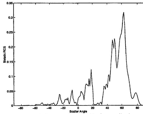
Figure 2. The vertically cross-polarized RCS of one realization versus the scatter angle \theta' \cos\phi' .
