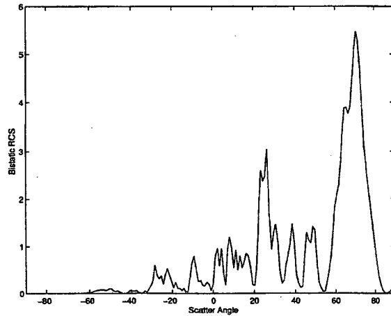
Figure 1. The vertically co-polarized RCS of one realization versus the scatter angle \theta^i \cos\phi^i .
