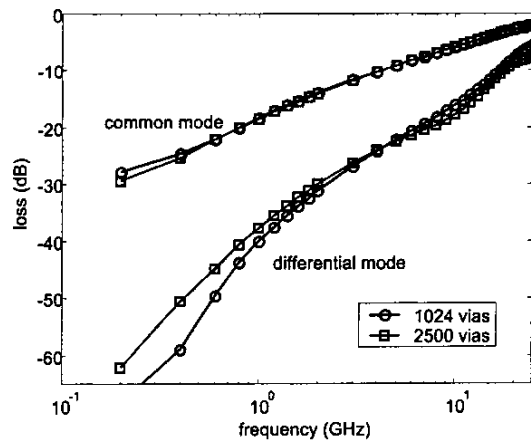
Fig. 5. Differential signaling with surrounding idle vias
