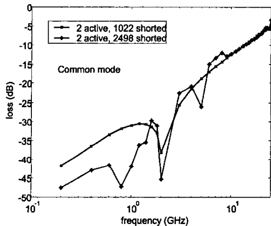
Fig. 7. Common mode with surrounding shorting vias
